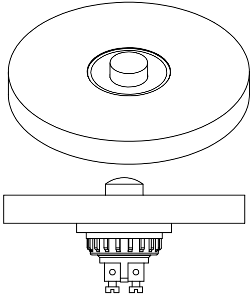
C size - 63.5mm diameter
