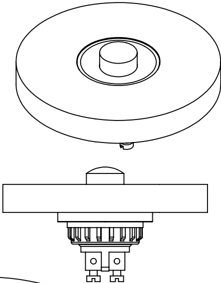
B size - 54mm Diameter
